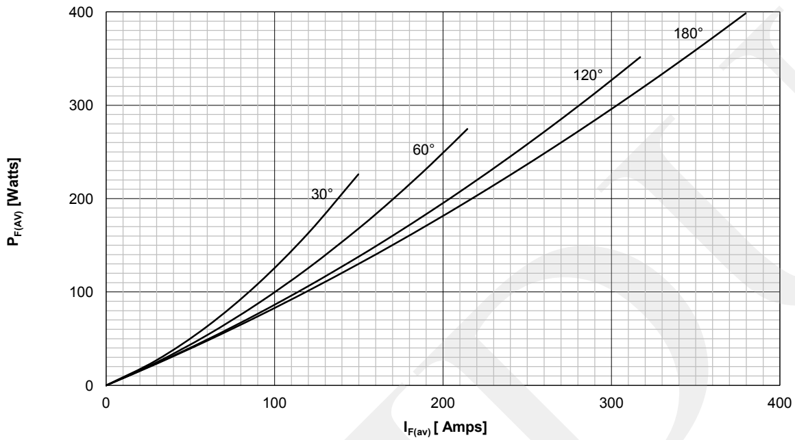
DISSIPATION CHARACTERISTICS PER ARM SINE WAVE
